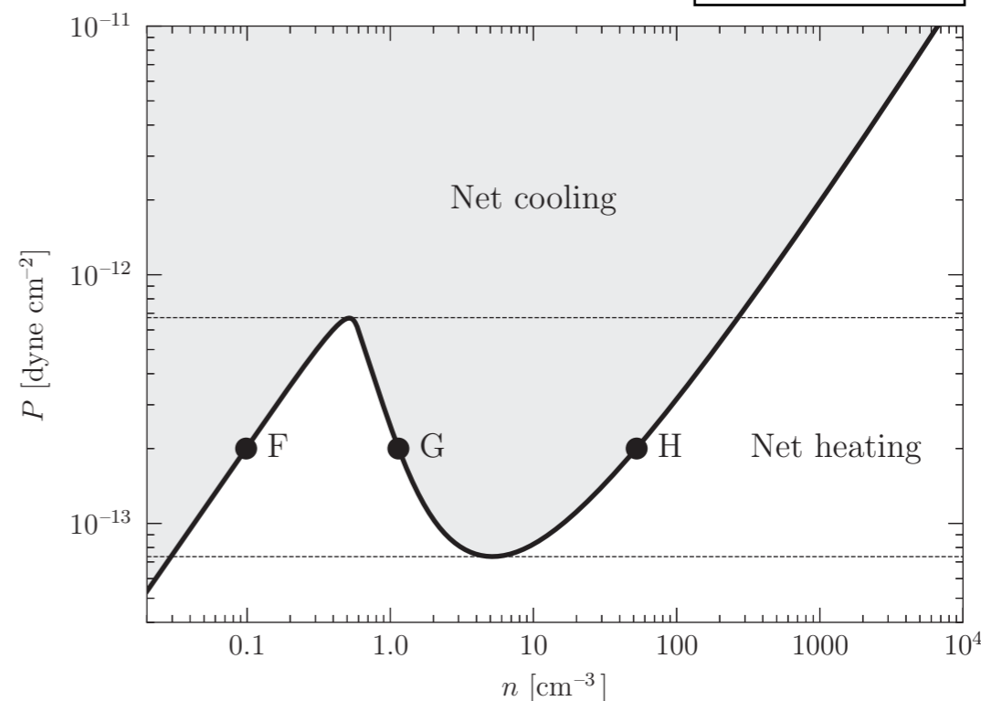
P vs n plane
