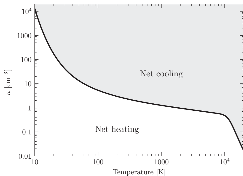
n vs T plane
