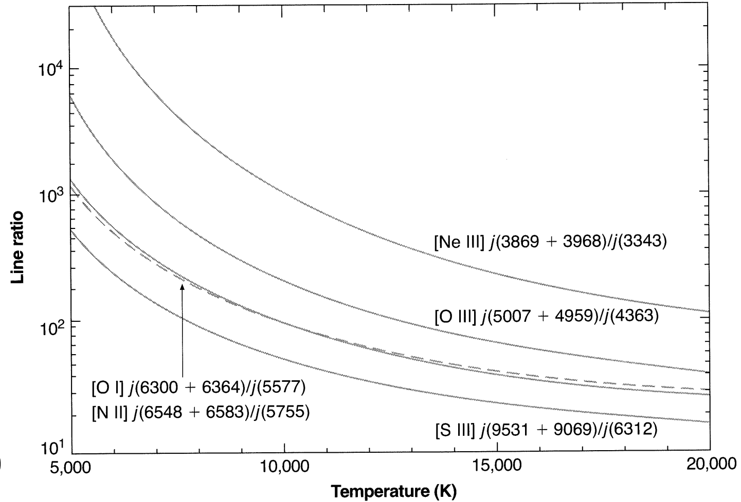
Figure 5.1 [Osterbrock]
