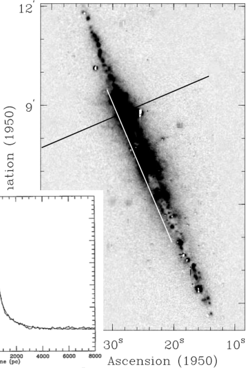
NGC 891 (Rand et al. 1998)
