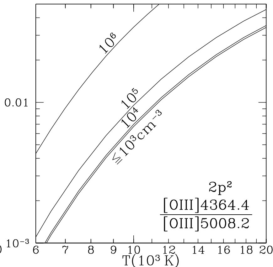
Figure 18.2 [Draine]
