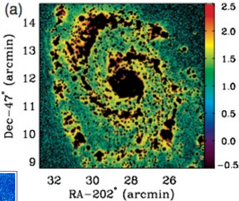
M 51 (Seon 2009)
