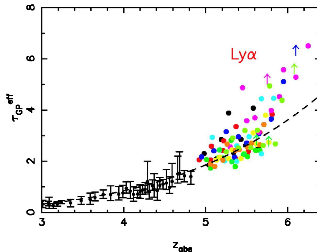
Ly \alpha optical depth as a function of redshift. [Fig 5, Fan et al. 2006, AJ, 132, 117] [See also Fan et al. 2006, AR&AA]
