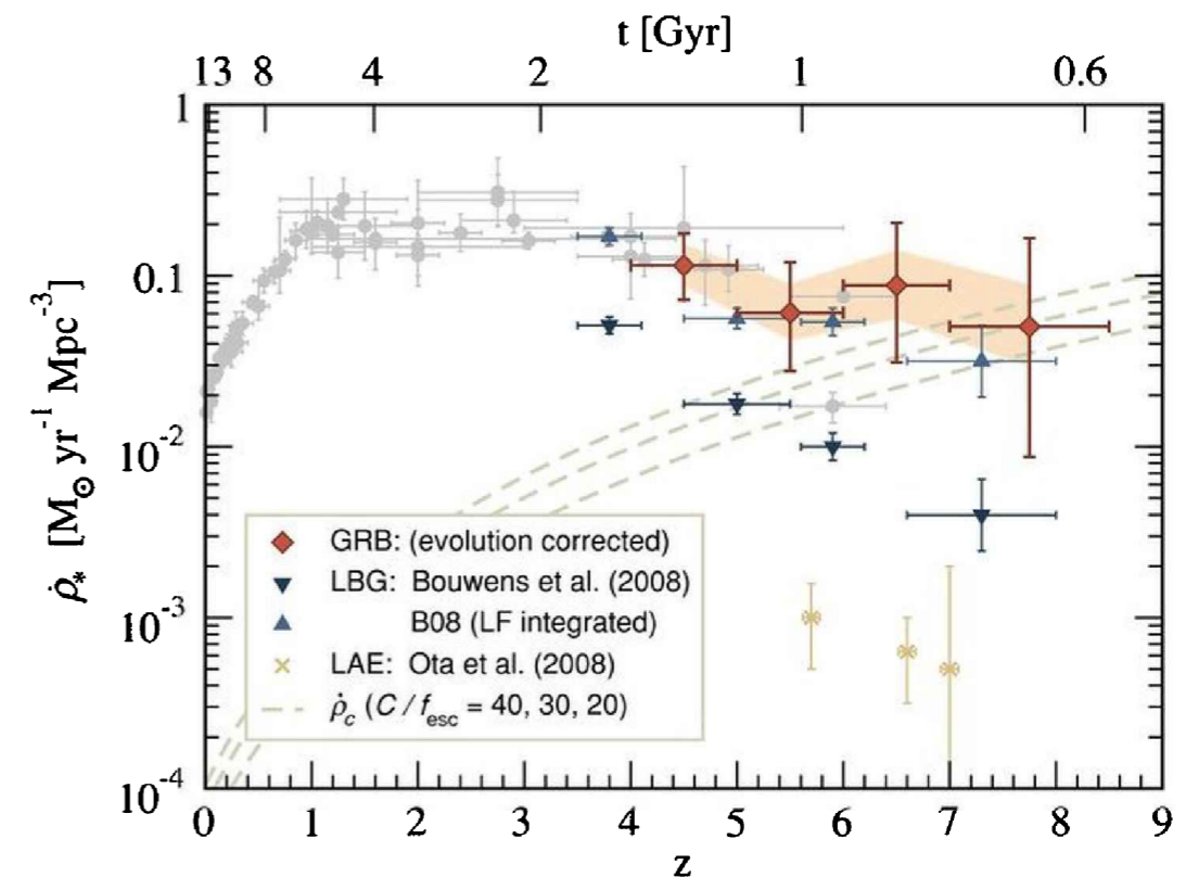
The cosmic star-formation rate using different traces (GRB = Gamma-Ray Bursts; LBG = Luminous Blue Galaxies; LAE = Lyman-Alpha Emitters) [Kistler et al. 2009; Fig 9.6 Ryden]
