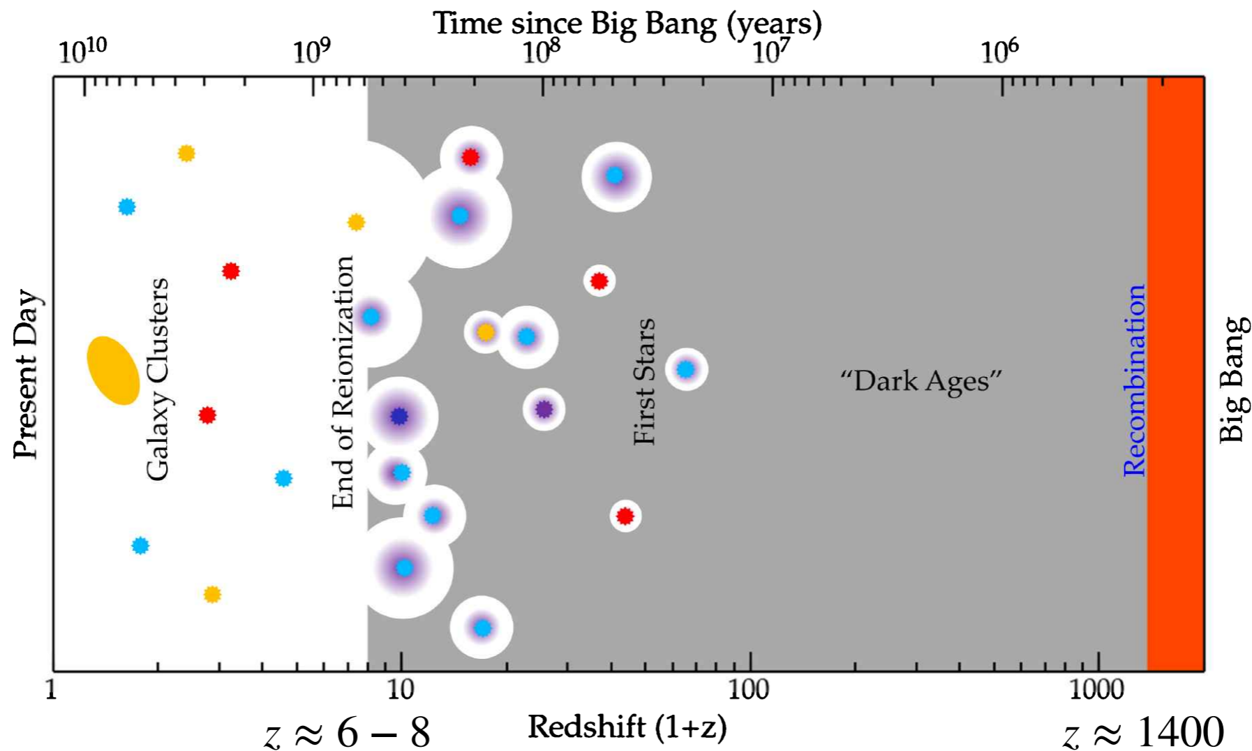
Schematic of the epoch of reionization [Barkana 2006; Fig 9.3 Ryden]
