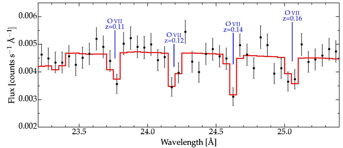
Simulated 700 ksec Chandra LETG/HRC spectrum of B2 1721+34 showing predicted WHIM O VII K \alpha absorption at redshifts of 0.11, 0.12, 0.14, and 0.16.
