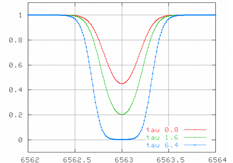
As N(\text{H I}) increases, the absorption line depth and width increase.
