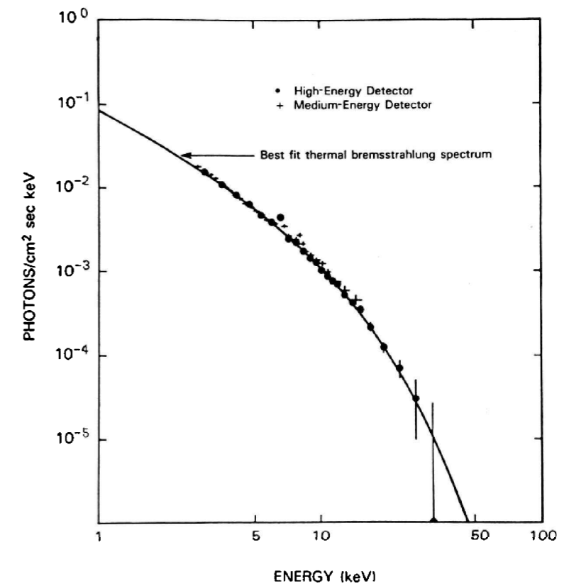
(top) X-ray image, (bottom) X-ray spectrum of the Coma Cluster [Henriksen & Mushotzky 1986]
