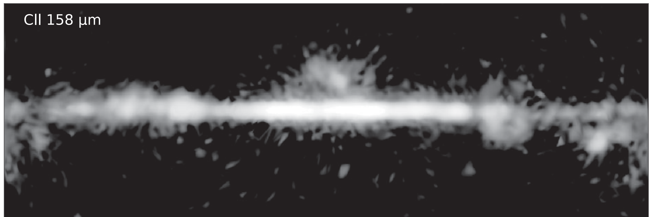
C II 158 \mu\text{m} line emission in the Galaxy. The map size is -180^\circ to 180^\circ in Galactic longitude and -60^\circ and 60^\circ in Galactic latitude. The data is from all-sky maps created by the Cosmic Microwave Background Explorer.
